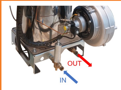
Inlet & Outlet M22 x 1.5
