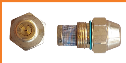
Fuel nozzle 2.25 60°
