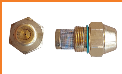
Fuel nozzle 2.5 60°
